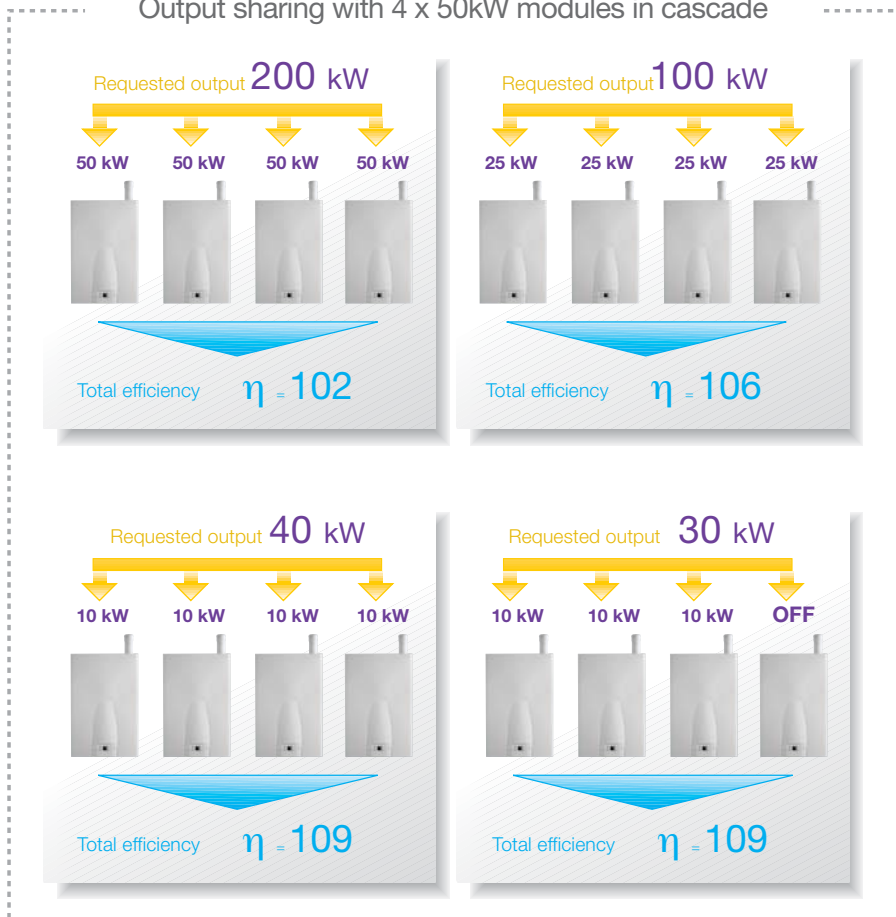
Output sharing with 4 x 50kW modules in cascade
